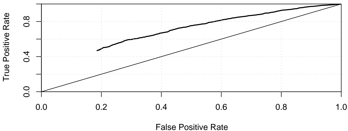
ROC Curve
